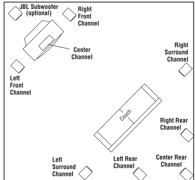
Figure 3. This figure shows an alternate layout, which may be more suitable for some rooms. Left/right rear channels are for a 7-channel system. The center rear channel is for a 6-channel system.
